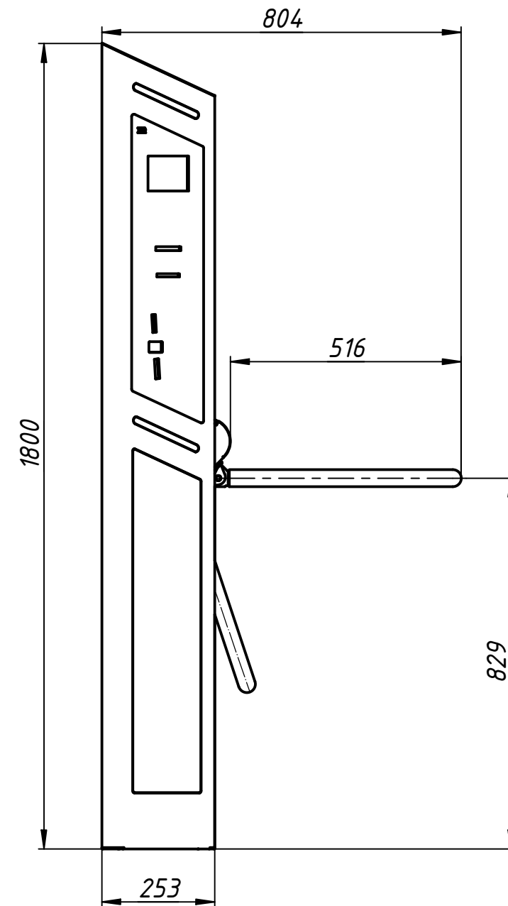
Installation tamplate
