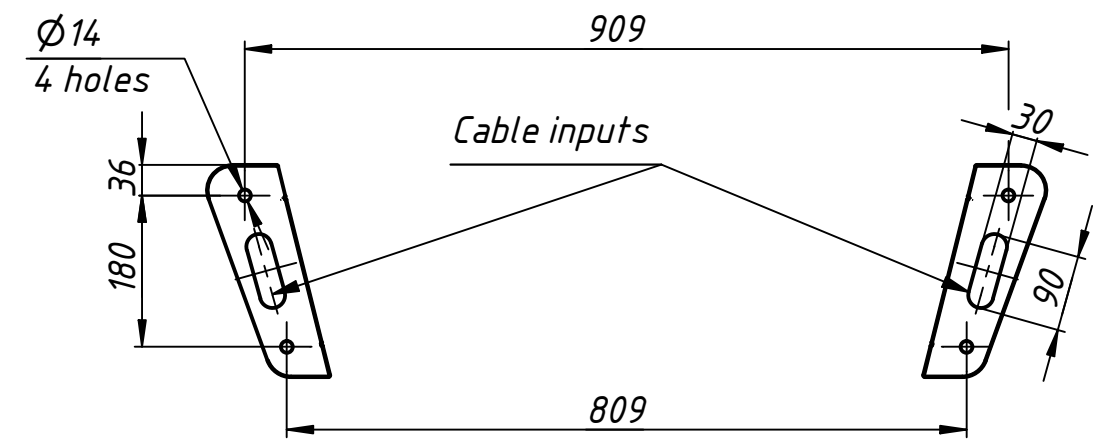
Installation tamplate
